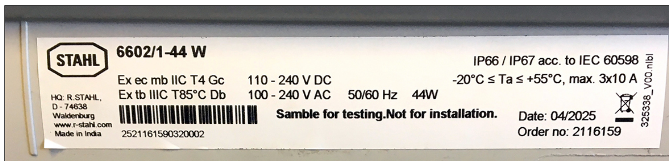
Figure 3.3: Test sample – ID label
