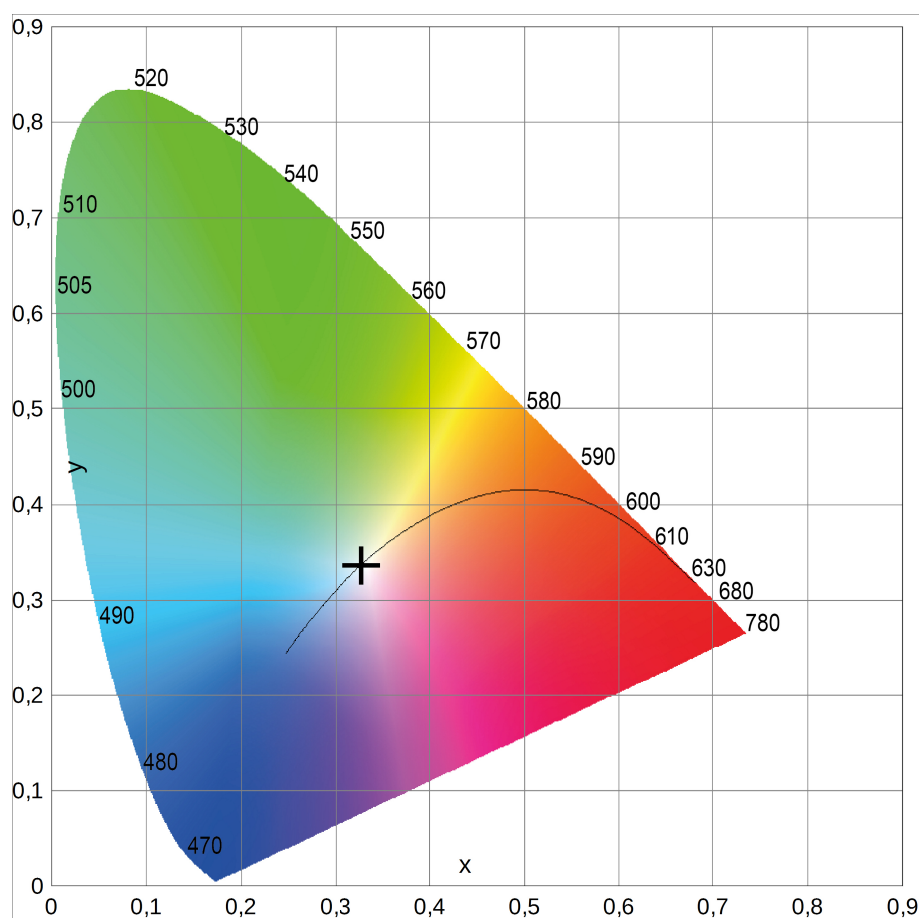
Diagram 6.2: Chromaticity diagram
