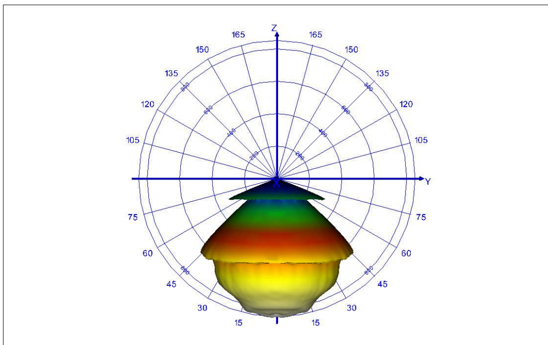
Figure 3: 3D - luminous intensity distribution
