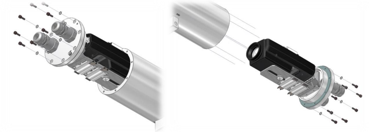
Fig. 6-3: Opening the ExCam T08-VAx.x.x.x camera
