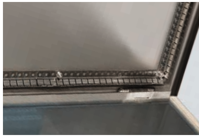
EMC contact spring prevents effects of electromagnetism
