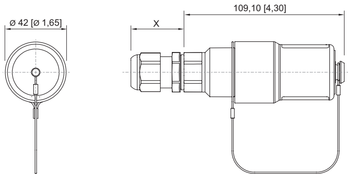
8595/1 Kupplung
