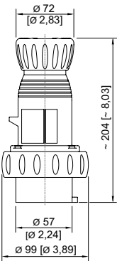
Stecker 4-polig
