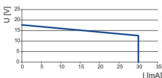
9475/32-08-52, 9475/33-08-50 output characteristic
