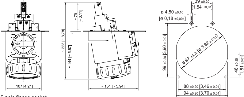
5-pole flange socket Clock hour position 2 h, 3 h, 4 h
