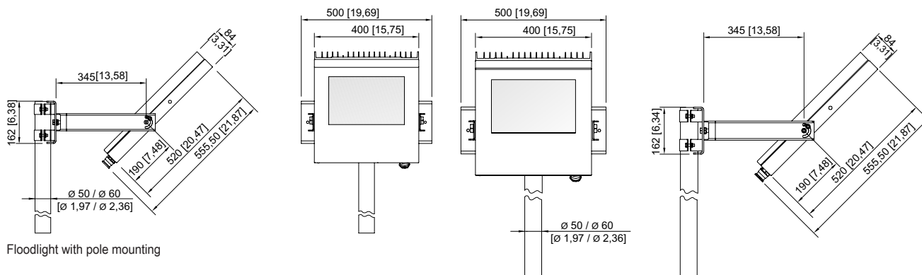
Mounting bracket
