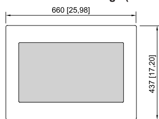
Panel mount front view
