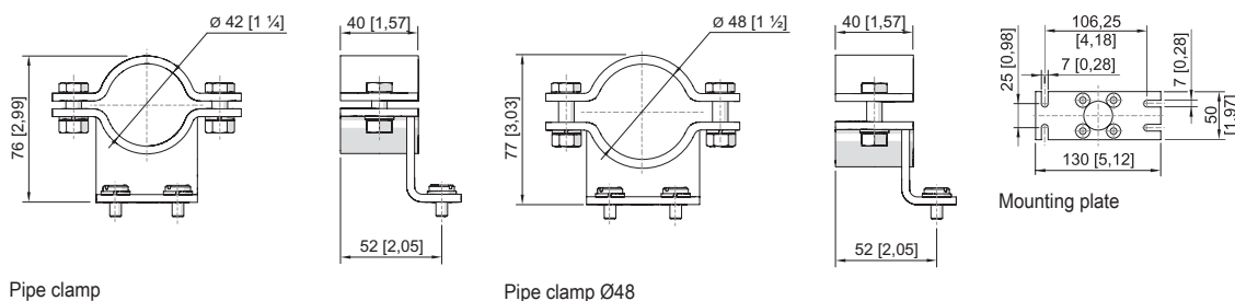
Pipe clamp
