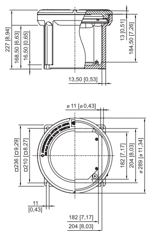
Size 4 enclosure without sight glass
