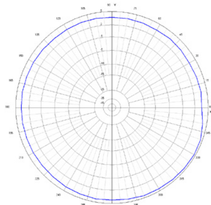
Radiation characteristics for 2.4 GHz Type 9790/1-2458-NT.-53
