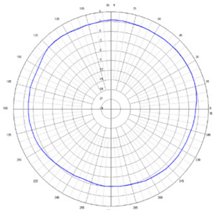
Radiation characteristics for 2.1 GHz Type 9790/1-0826-NTM-02
