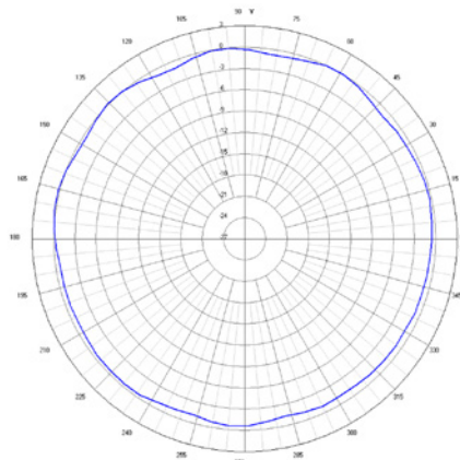
Radiation characteristics for 2.59 GHz Type 9790/1-0826-NTM-02
