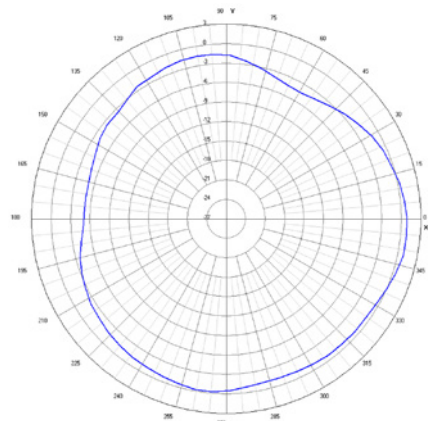
Radiation characteristics for 920 MHz Type 9790/1-0826-NTM-02
