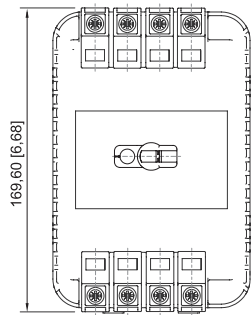
8530/1; 4 horizontal pitches
