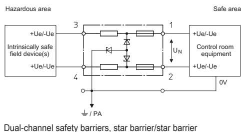
Dual-channel safety barriers, star barrier/star barrier
