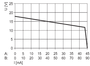
9175/0-14-11, 9176/0-14-00 output characteristic
