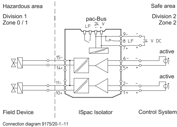
Connection diagram 9175/20-1.-11
