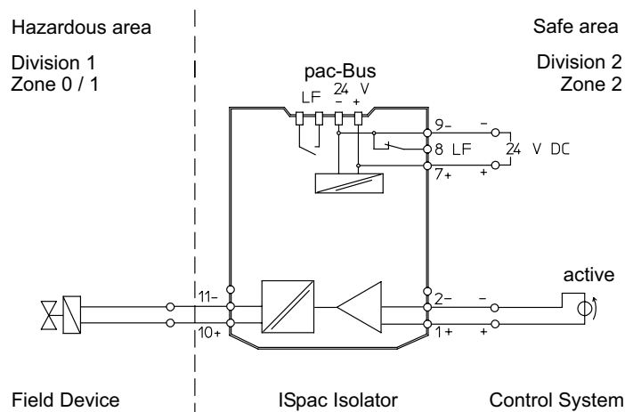
Connection diagram 9175/10-1.-11
