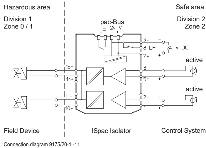
Connection diagram 9175/20-1.-11
