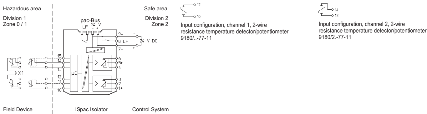
9180/2.-77-11 connection diagram
