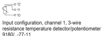
9180/2.-77-11 connection diagram
