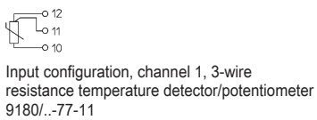
9180/2.-77-11 connection diagram
