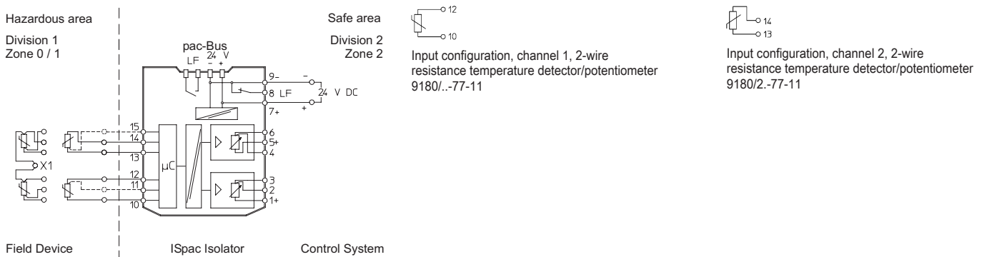
9180/2.-77-11 connection diagram
