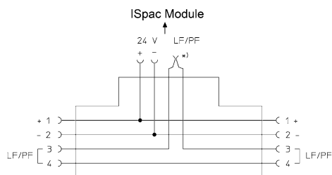
9194 connection diagram
