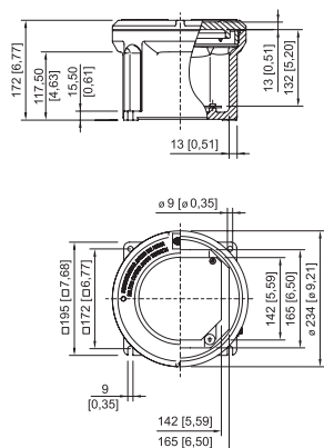
Size 3 enclosure without sight glass
