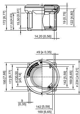
Size 3 enclosure with sight glass
