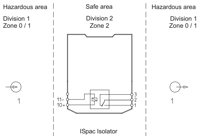
Connection diagram 9172/12-11-00
