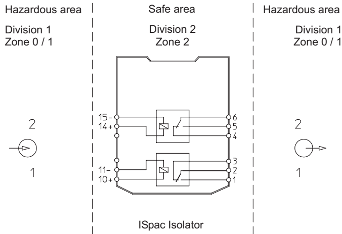
Connection diagram 9172/22-11-00
