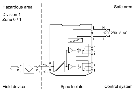
Connection diagram 9170/11-13-21
