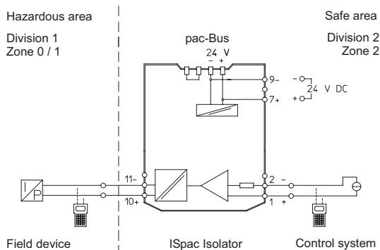
Connection diagram 9165/16-11-10
