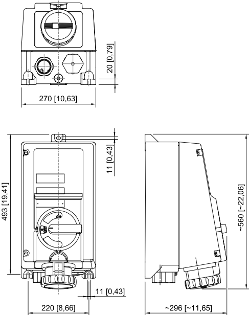
Wall-mounting socket
