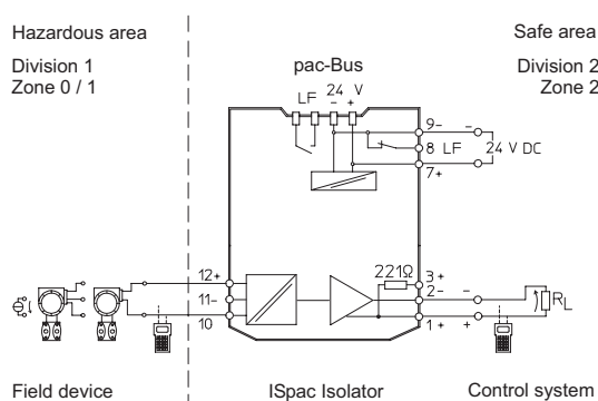
Connection diagram 9160/13-11-13
