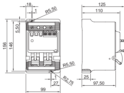
8562/54-2386-060, 2-pole with auxiliary contact and reset function
