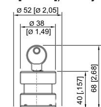
8003/...-006, 8003/...-009 mushroom stay-put button with key lock
