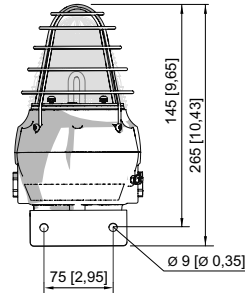
FX15 flashing beacon with L-bracket
