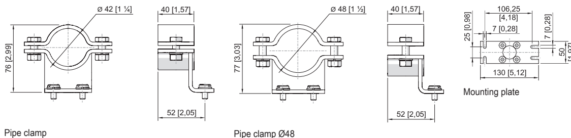
Pipe clamp
