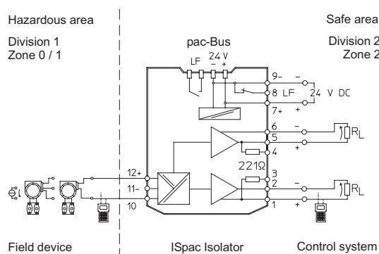
Connection diagram 9160/19-11-11
