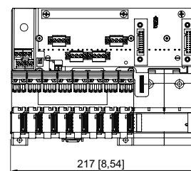
9419/04R bus-Carrier for 4 fieldbus segments
