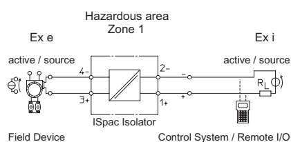
Connection diagram 9164/13-20-06
