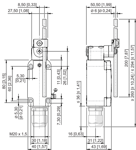
Rod lever 8074/2-DD-40
