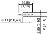
Straight actuator for safety switch
