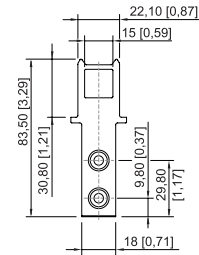
Safety switch 8070/2-1-AZ-U50
