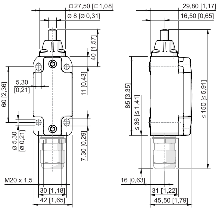
Domed plunger 8070/2-3-W-U60
