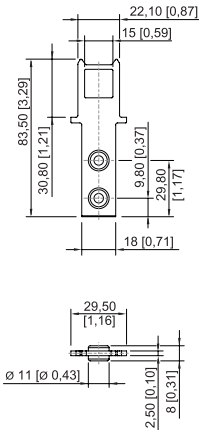
Straight actuator for safety switch
