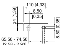
Wall mounting bracket fitted in mounting rail
