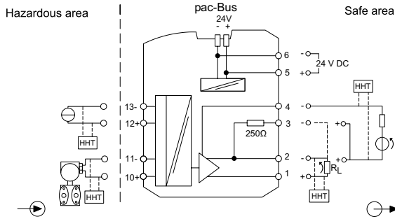
9260/13-11-10 connection diagram
