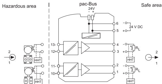
9260/23-11-10 connection diagram
