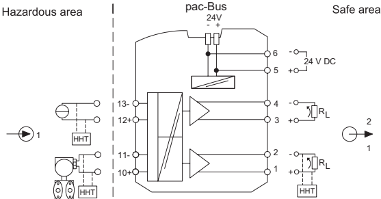
9260/19-11-10 connection diagram
