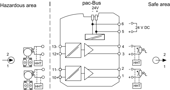
9260/23-11-10 connection diagram
