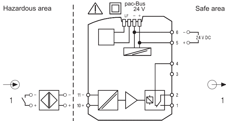
9270/11-16-14 connection diagram
