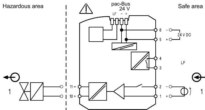
Connection diagram 9275/10-21-25-11
