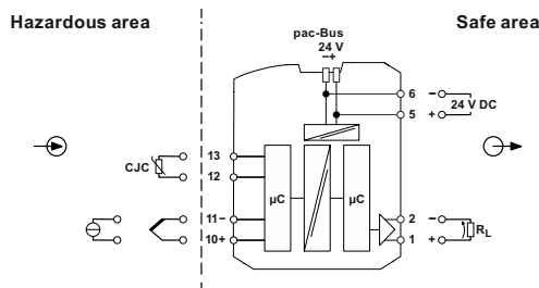
9282/12-51-16 connection diagram
