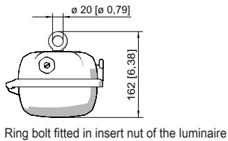
Ring bolt fitted in insert nut of the luminaire
